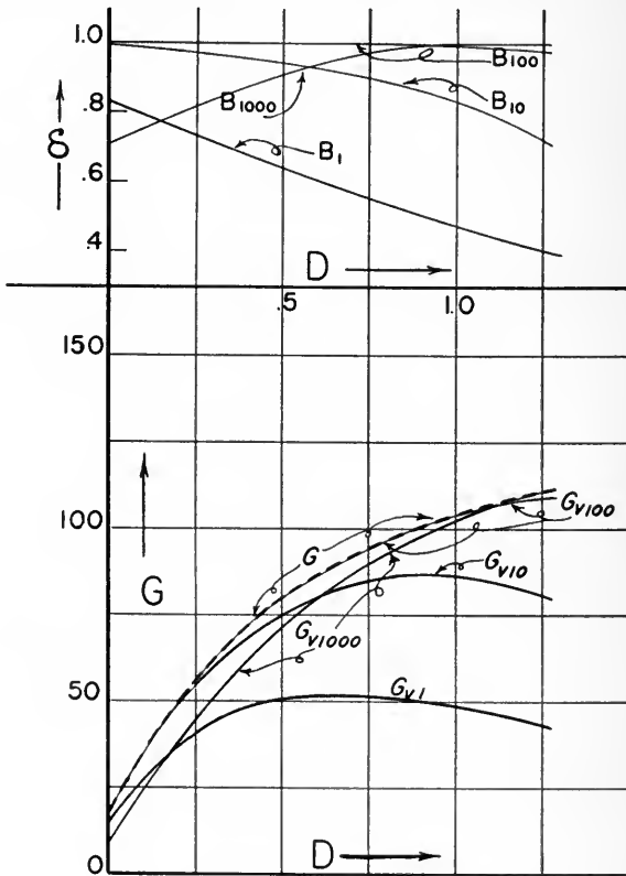
FIG. 13. The effect of field brightness upon the visually observed graininess. In the upper section \delta is plotted against D for B = 1 - 10^3 millilambert. In the lower section the G_1 curve of Fig. 9 (dashed) is transformed with the above \delta(D) into subjective graininess-density functions for different illuminations.
